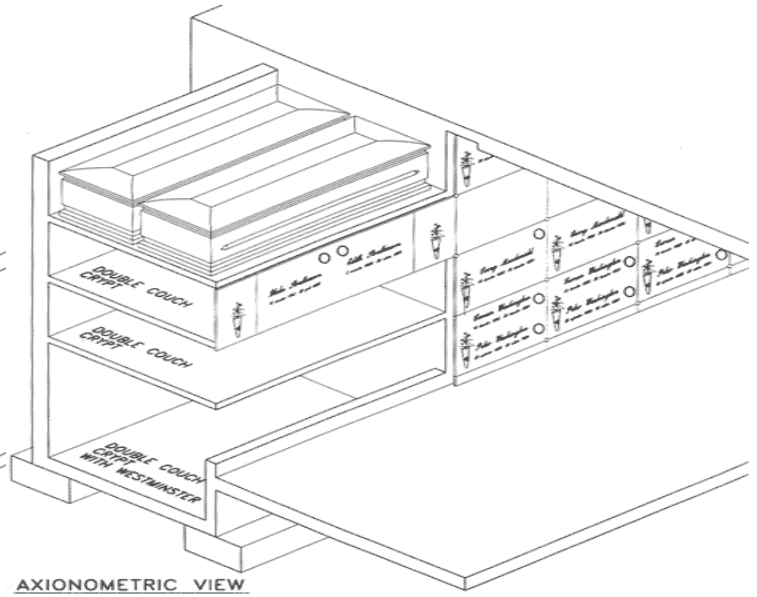
AXIONOMETRIC VIEW
