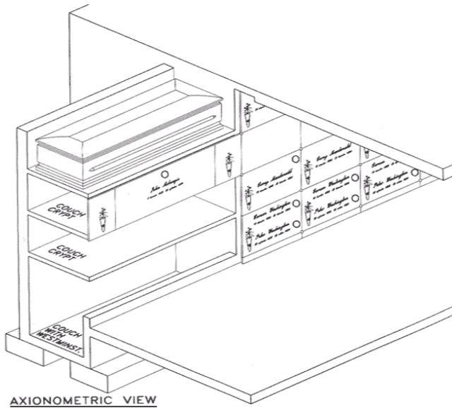
AXIONOMETRIC VIEW
