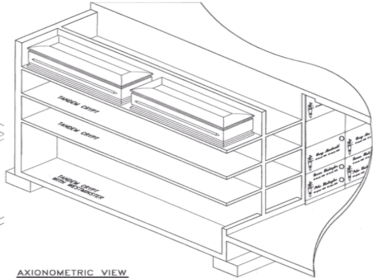
AXIONOMETRIC VIEW
