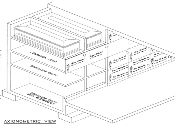
AXIONOMETRIC VIEW
