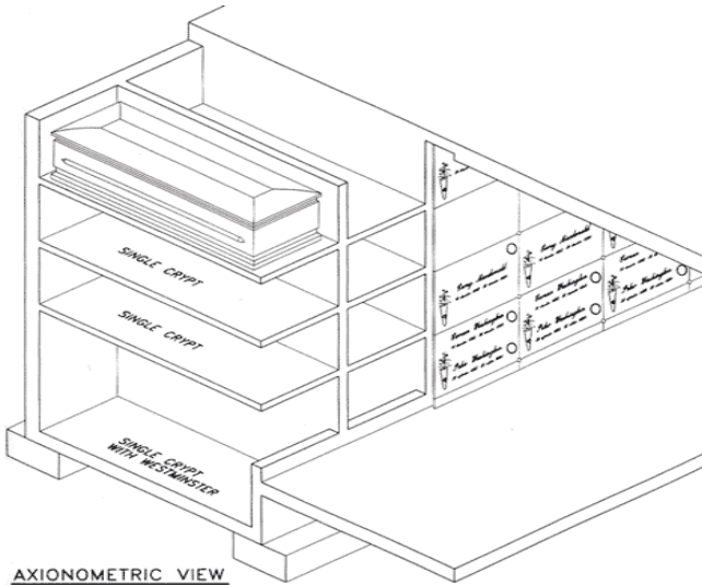
AXIONOMETRIC VIEW
